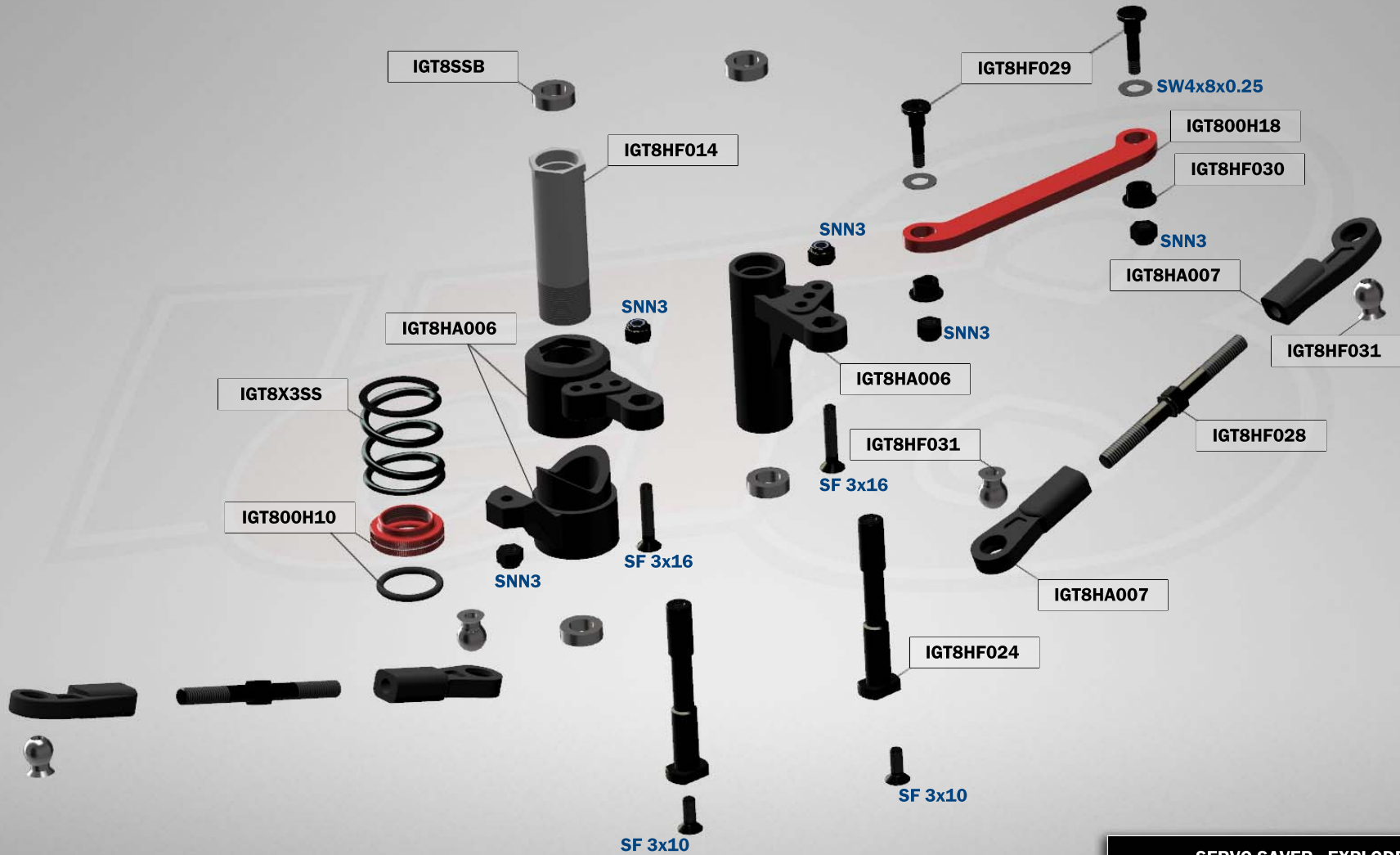
SERVO SAVER - EXPLODED VIEW
