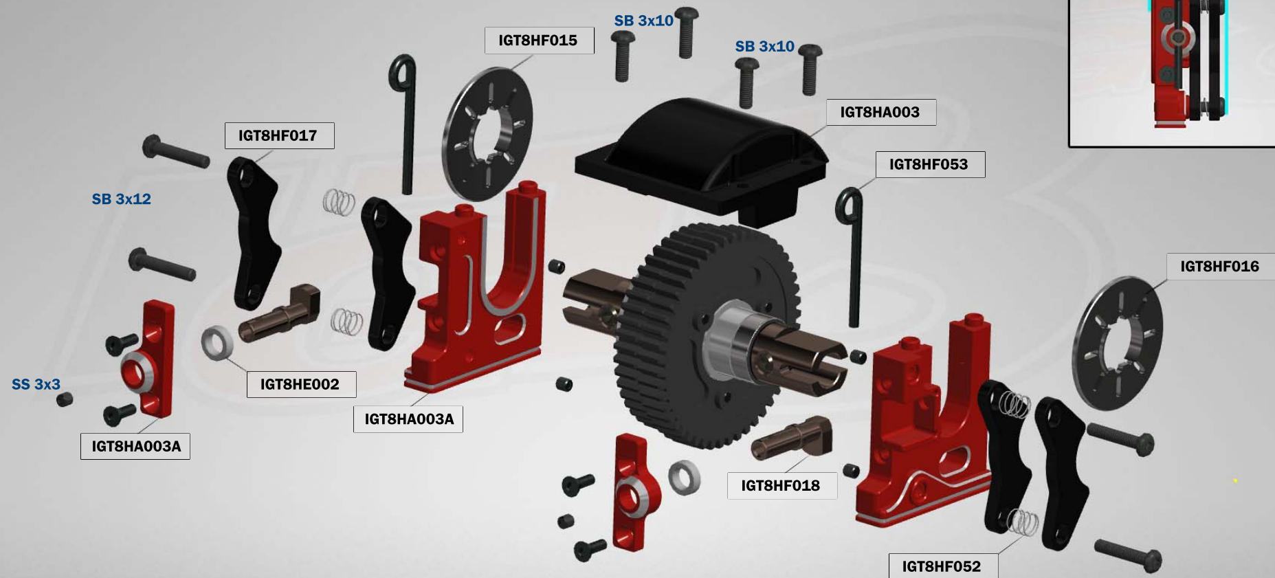
BRAKES - EXPLODED VIEW
